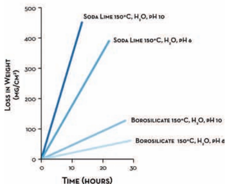
COMPARISON OF DEGRADATION OF BOROSILICATE VS. SODA LIME GLASS IN WATER
